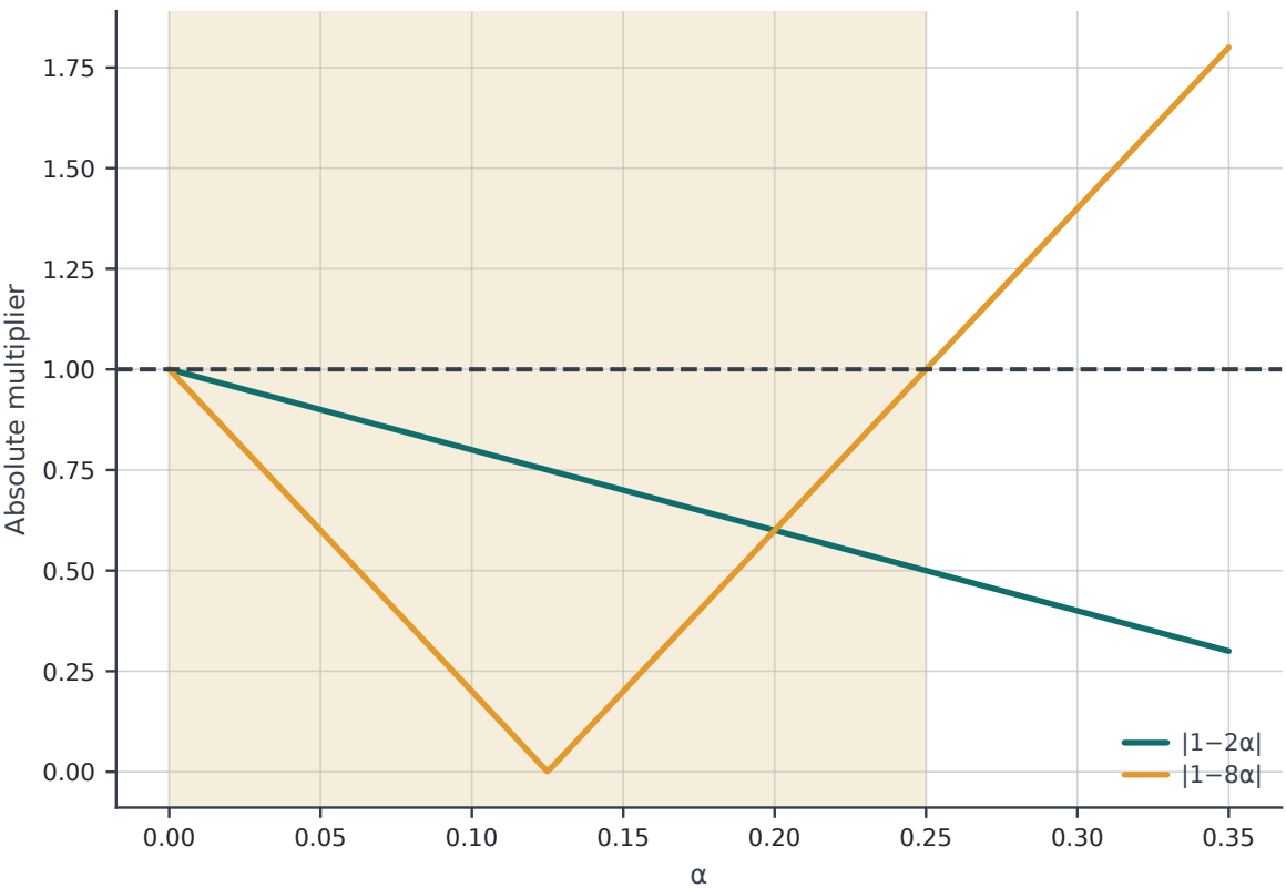
Contraction of the two error components
