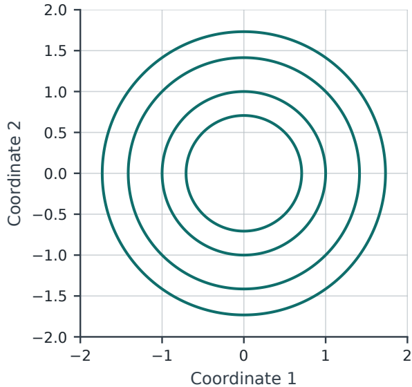
Scaled: z_1^2 + z_2^2
