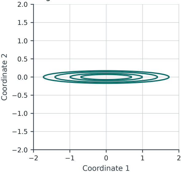
Original: e_1^2 + 100e_2^2
